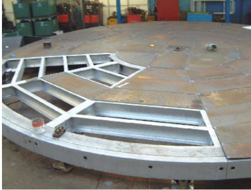
A 9-metre diameter mechanical commercial turntable undergoing construction prior to delivery
